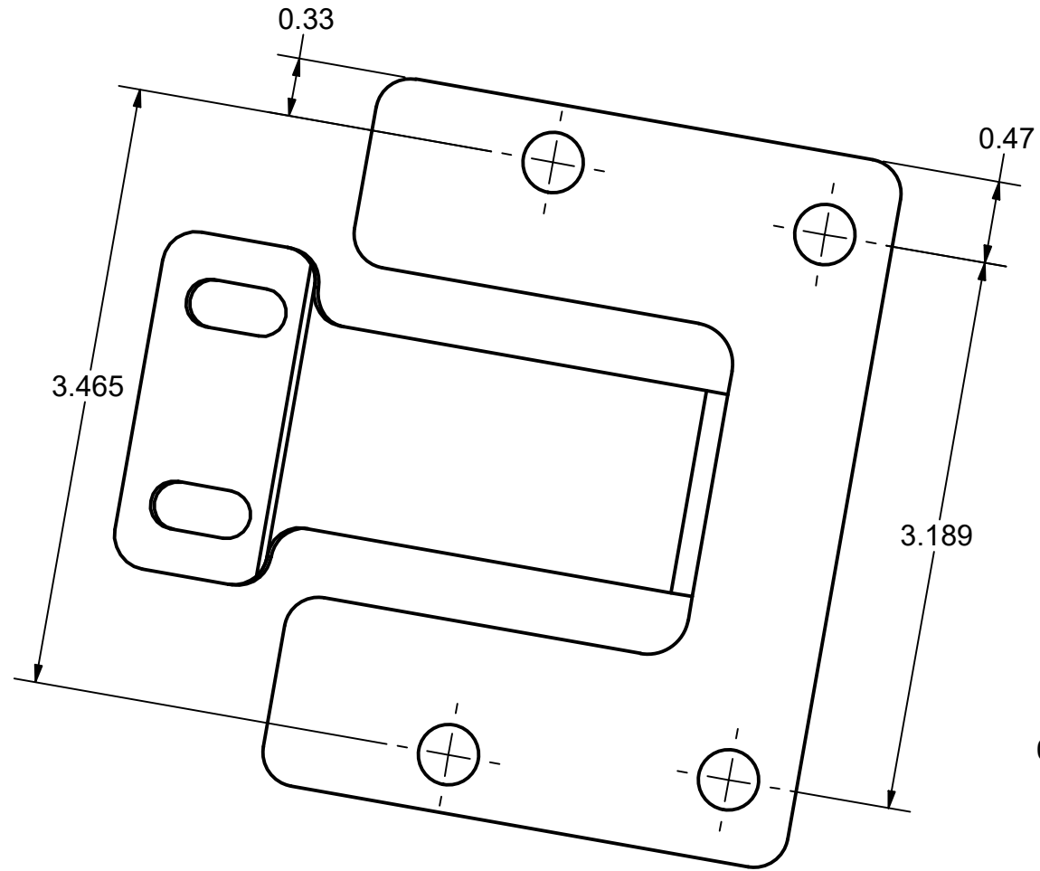
VIEW A-A SCALE 1 : 1
